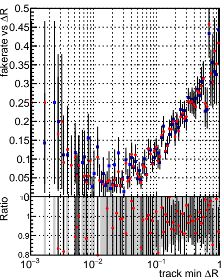
Fake rate vs \Delta R(\text{track, jet}) ■ DQM_mkFit_QCDHighPt_base ■ DQM_mkFit_QCDHighPt_retrain
