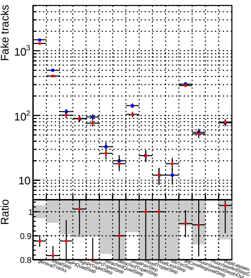
Number —●— DQM_mkFit_QCDHighPt_retrain
