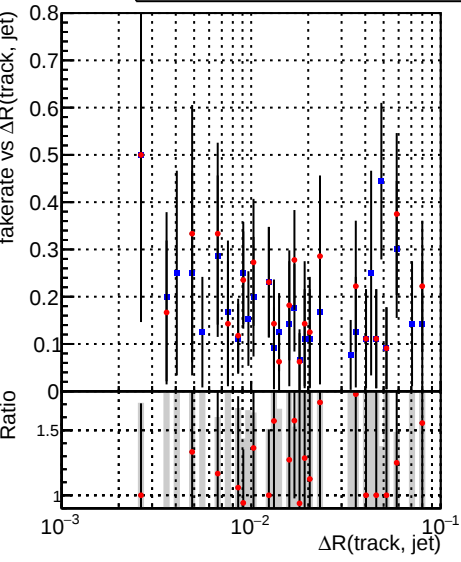
Legend: DQM_mkFit_QCDHighPt_base (blue dots), DQM_mkFit_QCDHighPt_retrain (red dots)
