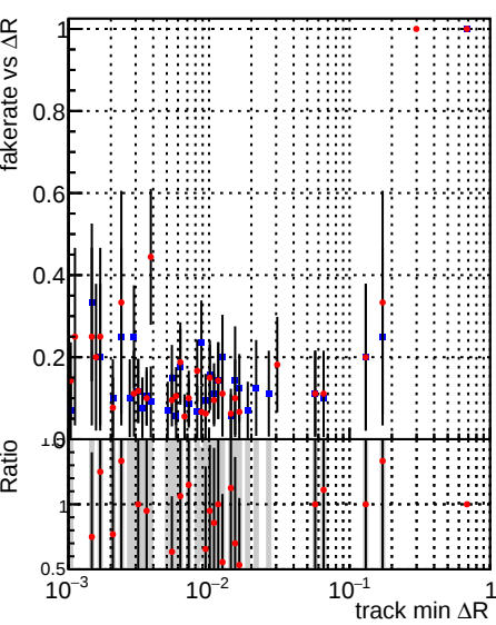
Legend: DQM_mkFit_QCDHighPt_base (blue dots), DQM_mkFit_QCDHighPt_retrain (red dots)
