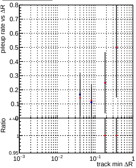
Legend: DQM_mkFit_QCDHighPt_base (blue dots), DQM_mkFit_QCDHighPt_retrain (red dots)
