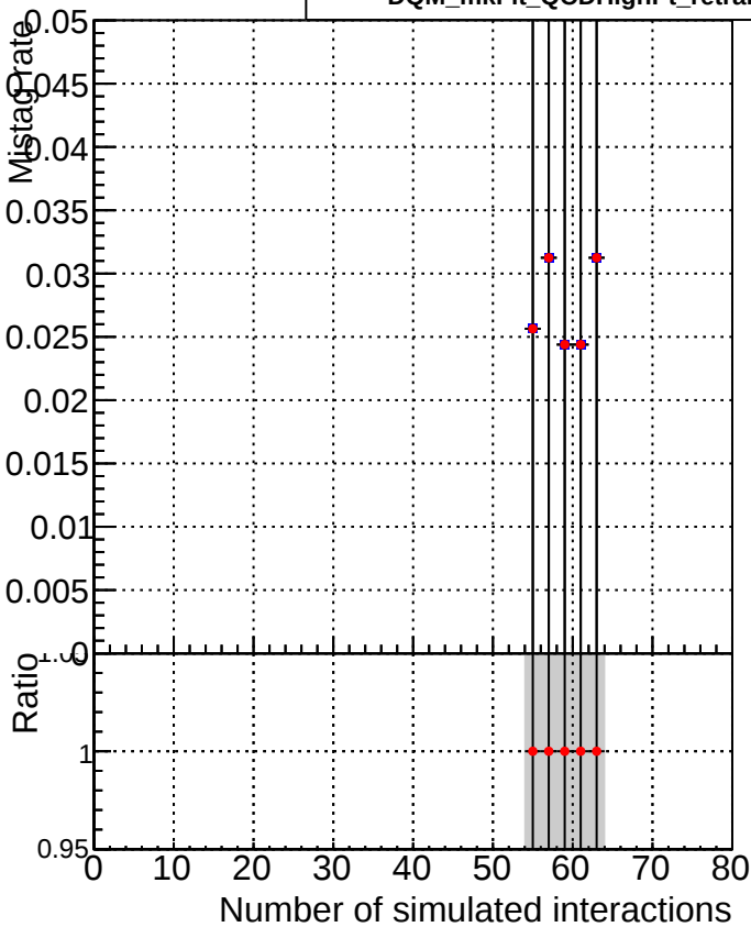
—•— DQM_mkFit_QCDHighPt_base —•— DQM_mkFit_QCDHighPt_retrain
