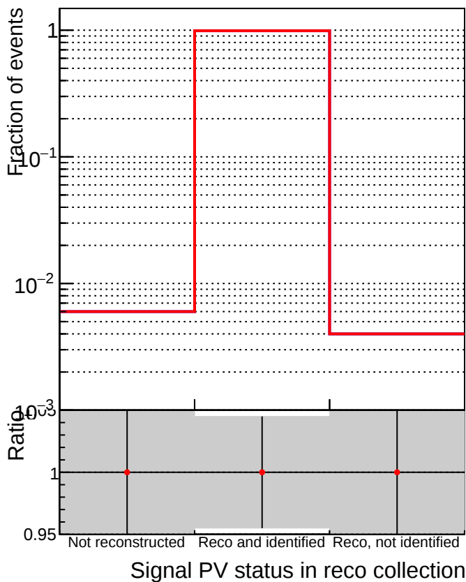
—•— DQM_mkFit_QCDHighPt_base —•— DQM_mkFit_QCDHighPt_retrain
