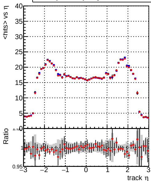
— DQM_mkFit_QCDHighPt_base — DQM_mkFit_QCDHighPt_retrain
