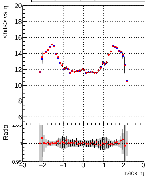
— DQM_mkFit_QCDHighPt_base — DQM_mkFit_QCDHighPt_retrain mean hits vs \eta
