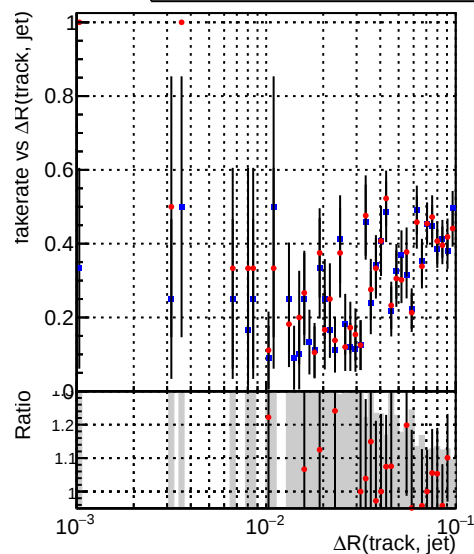
—●— DQM_mkFit_QCDHighPt_base —●— DQM_mkFit_QCDHighPt_retrain
