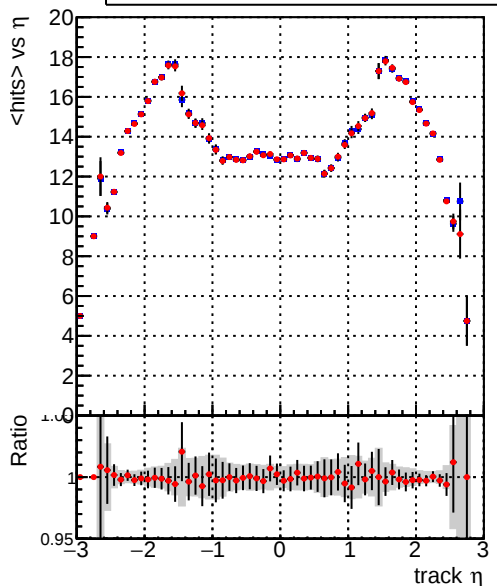
mean hits — DQM_mkFit_QCDHighPt_base — DQM_mkFit_QCDHighPt_retrain
