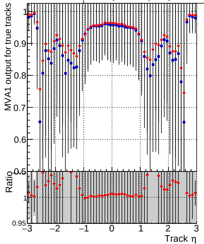
MVA1 of associated tracks (recoToSim) vs. track \eta Legend: ■ DQM_mkFit_QCDHighPt_base ● DQM_mkFit_QCDHighPt_retrain
