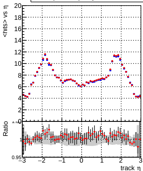
mean hits vs \eta — DQM_mkFit_QCDHighPt_base — DQM_mkFit_QCDHighPt_retrain
