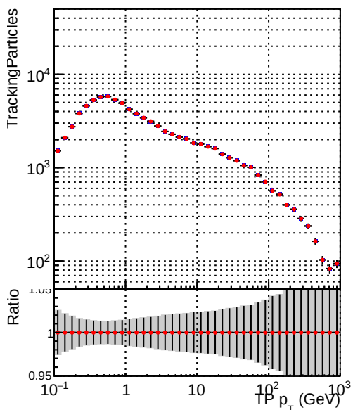
—•— DQM_mkFit_QCDHighPt_base —•— DQM_mkFit_QCDHighPt_retrain
