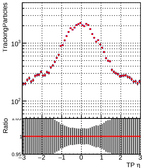
—•— DQM_mkFit_QCDHighPt_base —•— DQM_mkFit_QCDHighPt_retrain
