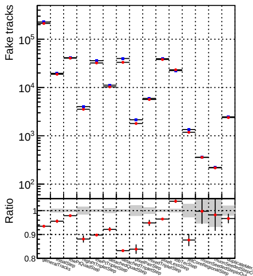
Number Model 1 DQM_mkFit_QCDHighPt_retrain
