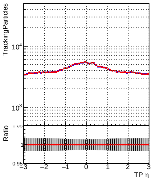
—•— DQM_mkFit_QCDHighPt_base - - - DQM_mkFit_QCDHighPt_retrain
