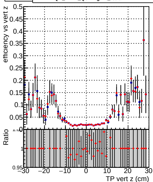
Efficiency —●— DQM_mkFit_QCDHighPt_retrain
