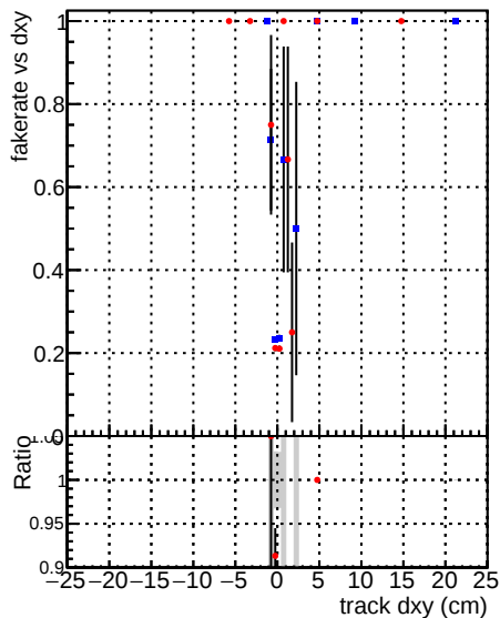
—●— DQM_mkFit_QCDHighPt_base —●— DQM_mkFit_QCDHighPt_retrain
