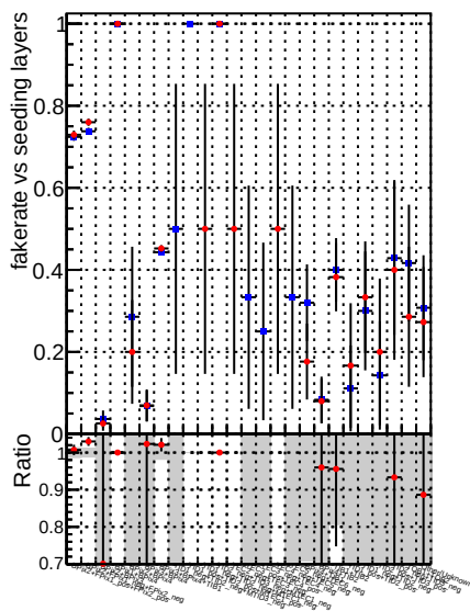
Fake rate vs. seeders
