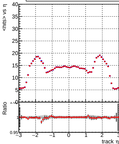
— DQM_mkFit_QCDHighPt_base — DQM_mkFit_QCDHighPt_retrain mean hits
