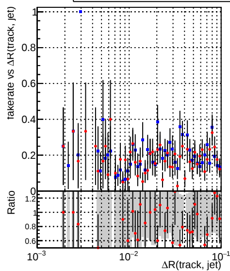
—●— DQM_mkFit_QCDHighPt_base —●— DQM_mkFit_QCDHighPt_retrain
