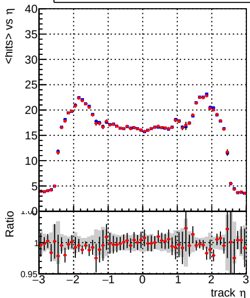
— DQM_mkFit_QCDHighPt_base — DQM_mkFit_QCDHighPt_retrain mean hits
