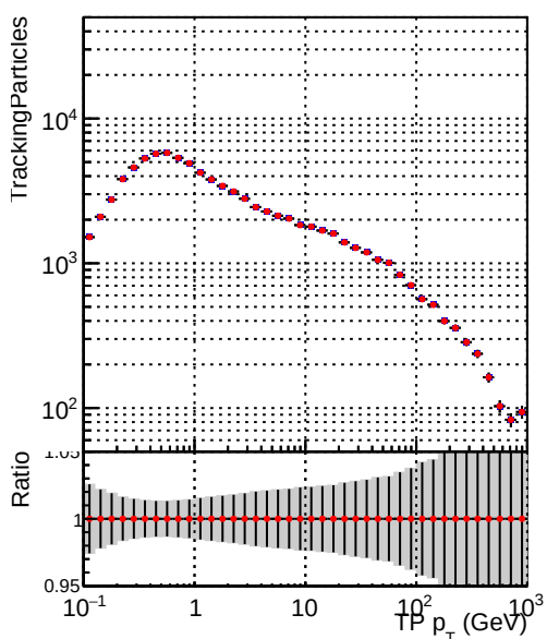
—•— DQM_mkFit_QCDHighPt_base —•— DQM_mkFit_QCDHighPt_retrain
