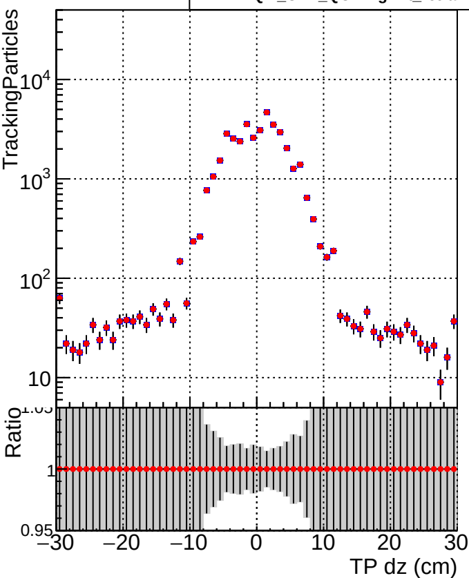
■ DQM_CKF_QCDHighPt_base ● DQM_CKF_QCDHighPt_retrain
