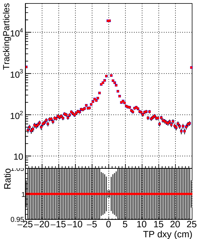
■ DQM_CKF_QCDHighPt_base ● DQM_CKF_QCDHighPt_retrain
