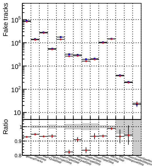
Number —●— DQM_CKF_QCDHighPt_retrain
