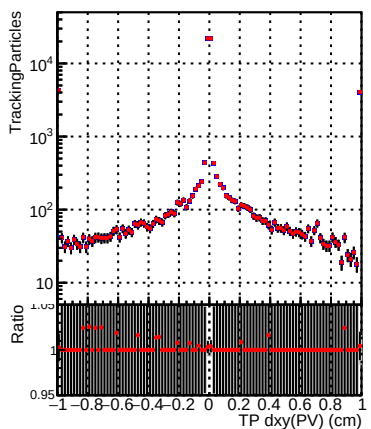
N of sim — DQM_CKF_QCDHighPt_retrain
