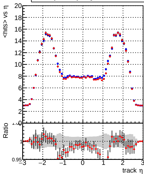
mean hit DQM_CKF_QCDHighPt_base DQM_CKF_QCDHighPt_retrain
