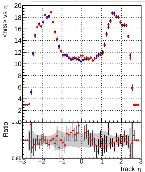
mean hits vs \eta Legend: DQM_CKF_QCDHighPt_base (blue line), DQM_CKF_QCDHighPt_retrain (red line)
