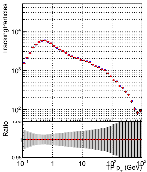
—•— DQM_CKF_QCDHighPt_base —•— DQM_CKF_QCDHighPt_retrain
