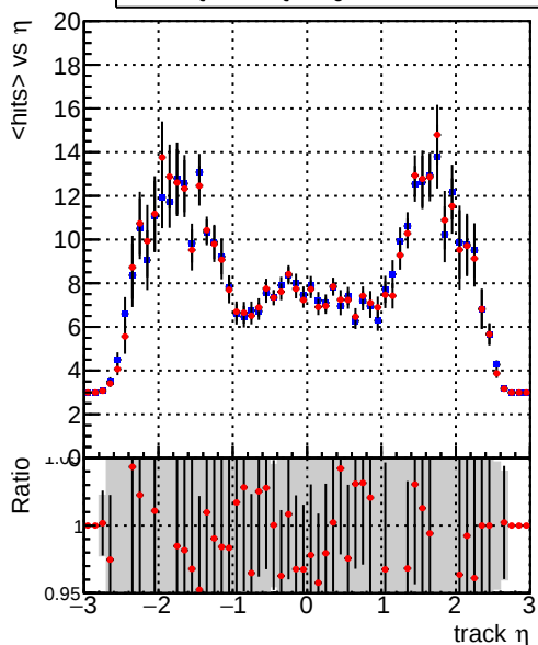
mean hits — DQM_CKF_QCDHighPt_base — DQM_CKF_QCDHighPt_retrain
