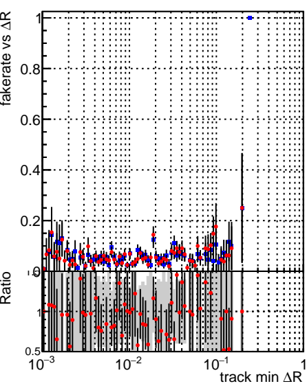
Fake rate vs \Delta R(\text{track, jet}) ■ DQM_CKF_QCDHighPt_base ● DQM_CKF_QCDHighPt_retrain
