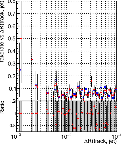
Fake rate vs \Delta R(\text{track, jet}) ■ DQM_CKF_QCDHighPt_base ● DQM_CKF_QCDHighPt_retrain
