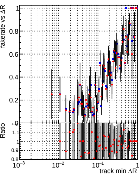
Fake rate vs \Delta R(\text{track, jet}) Legend: DQM_CKF_QCDHighPt_base (blue dots) DQM_CKF_QCDHighPt_retrain (red dots)
