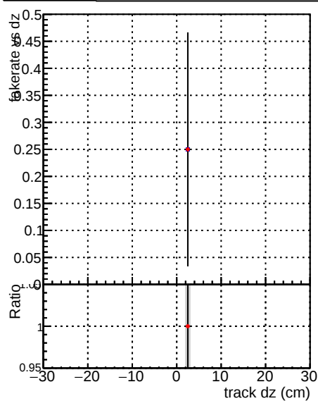
—●— DQM CKF QCDHighPt_base —●— DQM CKF QCDHighPt_retrain
