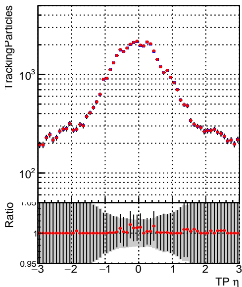
—•— DQM_CKF_QCDHighPt_base —•— DQM_CKF_QCDHighPt_retrain
