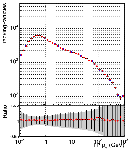
—•— DQM_CKF_QCDHighPt_base —•— DQM_CKF_QCDHighPt_retrain
