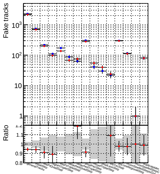
Number —●— DQM_CKF_QCDHighPt_retrain
