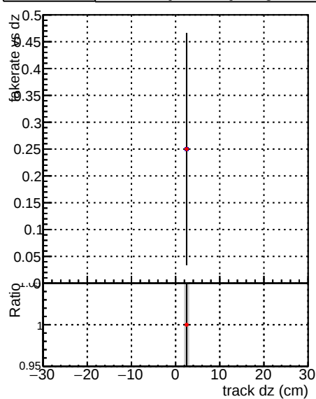
—●— DQM_CKF_QCDHighPt_base —●— DQM_CKF_QCDHighPt_retrain
