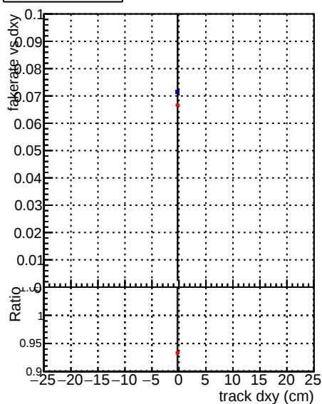
—●— DQM_CKF_QCDHighPt_base —●— DQM_CKF_QCDHighPt_retrain
