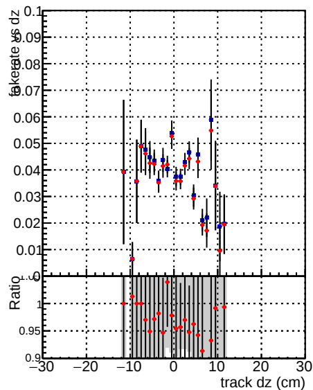
Fake rate vs dz —●— DQM CKF QCDHighPt_base —●— DQM CKF QCDHighPt_retrain
