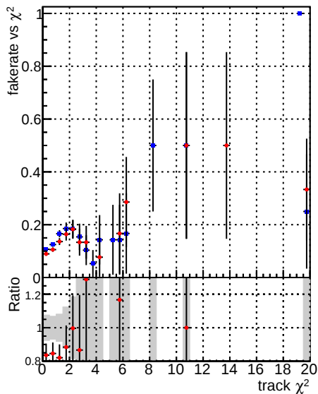
Fake rate vs. —* DQM CKF QCDHighPt_base —* DQM CKF QCDHighPt_retrain
