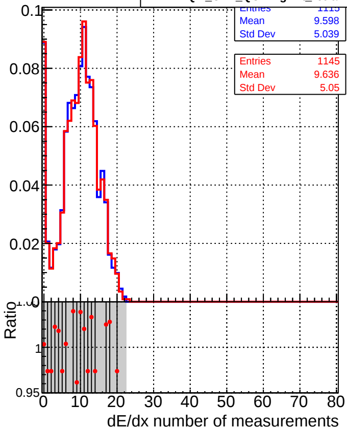
■ DQM_CKF_QCDHighPt_base ● DQM_CKF_QCDHighPt_retrain
