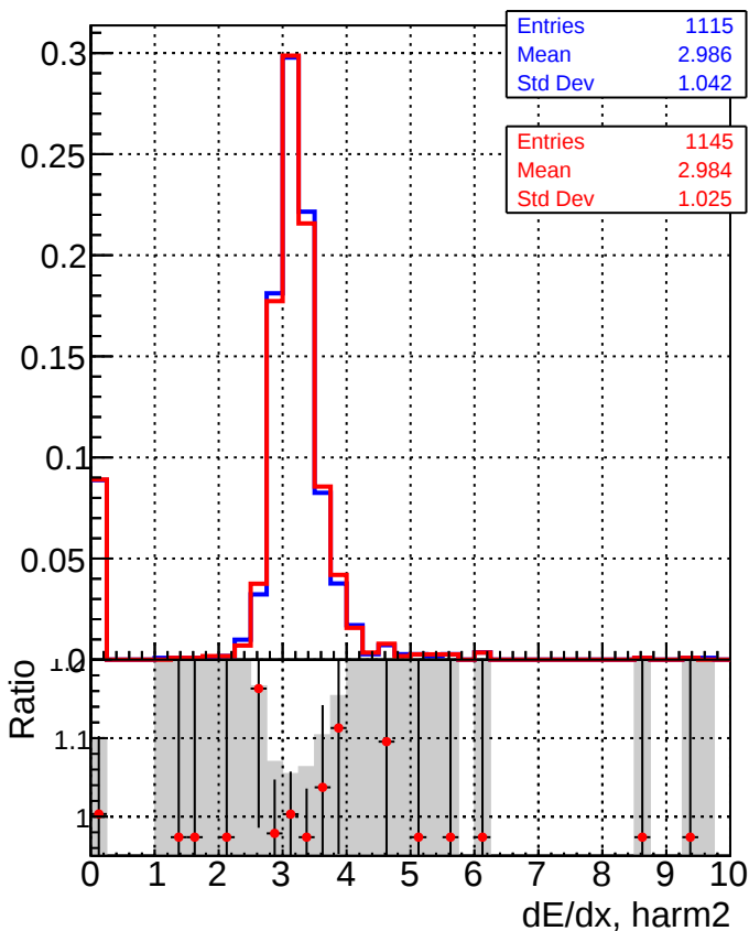
■ DQM_CKF_QCDHighPt_base ● DQM_CKF_QCDHighPt_retrain
