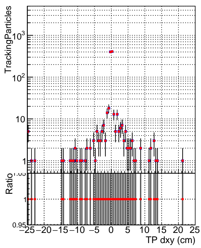
N of simulated track DQM_CKF_QCDHighPt_base DQM_CKF_QCDHighPt_retrain
