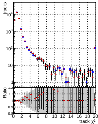
N of reco track vs. \chi^2 —●— DQM_CKF_QCDHighPt_base —●— DQM_CKF_QCDHighPt_retrain
