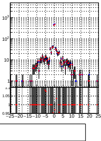
N of associated tracks (simToReco) vs dxy(PV)
