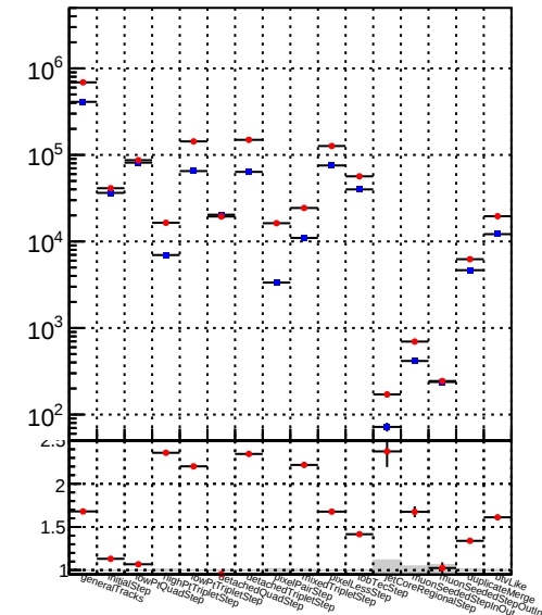
Number —●— DQM_BDT_mkFit
