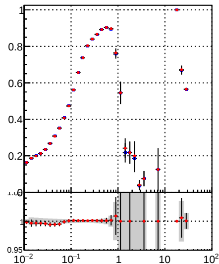
—•— DQM_mkFit —•— DQM_BDT_mkFit
