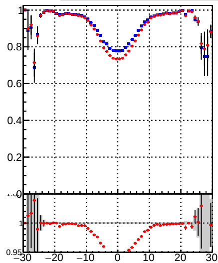
—•— DQM_mkFit —•— DQM_BDT_mkFit
