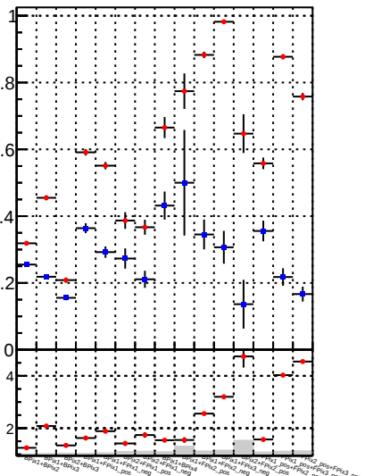
Fake rate vs. —•— DQM_mkFit —•— DQM_BDT_mkFit
