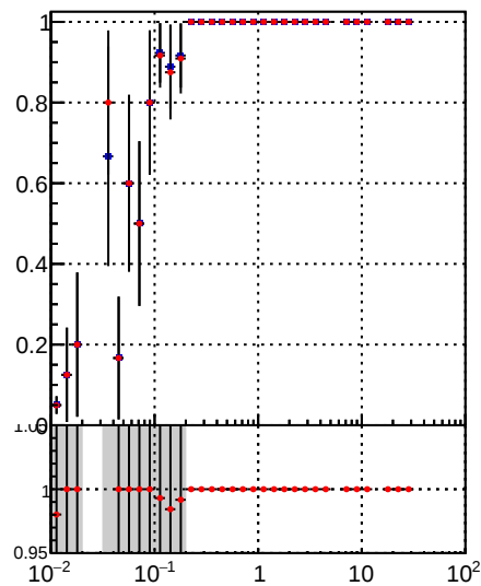
Fake rate vs v DQM_mkFit DQM_BDT_mkFit
