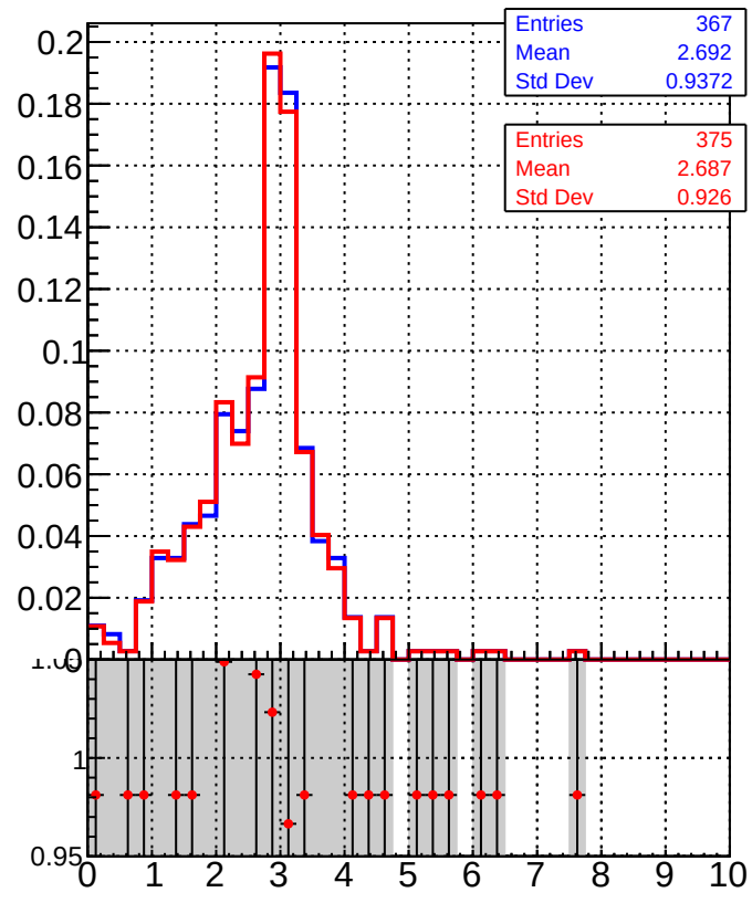
Legend: DQM_mkFit (Blue line with square markers), DQM_BDT_mkFit (Red line with square markers)
