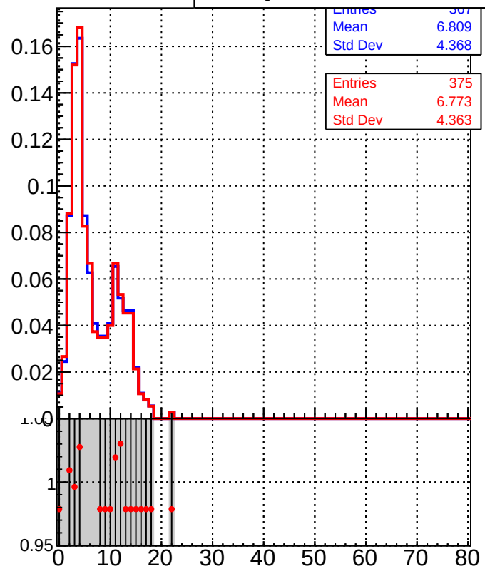
Legend: DQM_mkFit (Blue line with square markers), DQM_BDT_mkFit (Red line with square markers)
