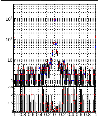
—•— DQM_mkFit —•— DQM_BDT_mkFit
