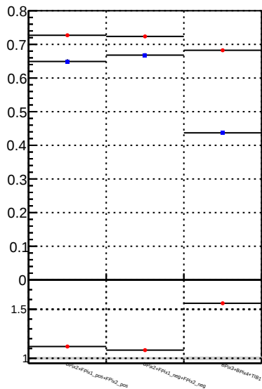
Fake rate vs. —●— DQM_mkFit —●— DQM_BDT_mkFit
