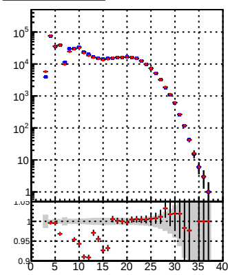
—•— DQM_mkFit —•— DQM_BDT_mkFit
