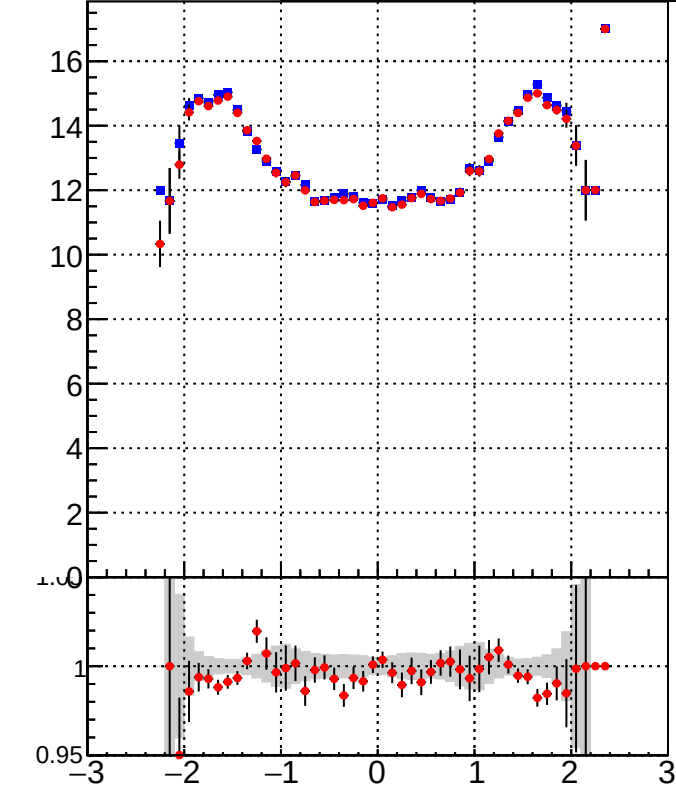
mean # STRIP hits v
