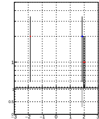
N of associated (recoToSim) tracks vs \eta ◆ DQM_mkFit + DQM_BDT_mkFit
